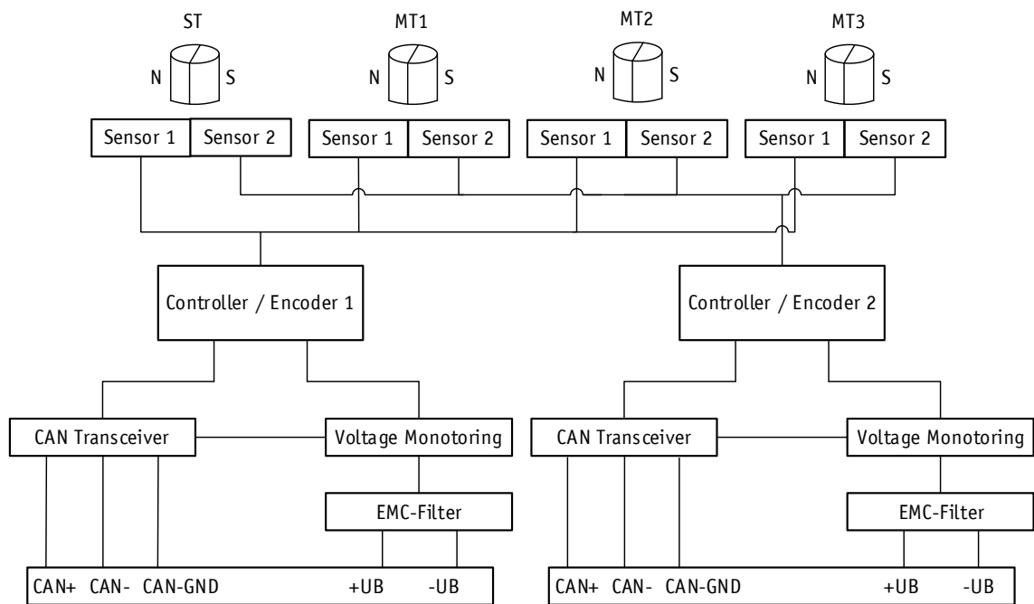
Fig. 1: Block diagram
