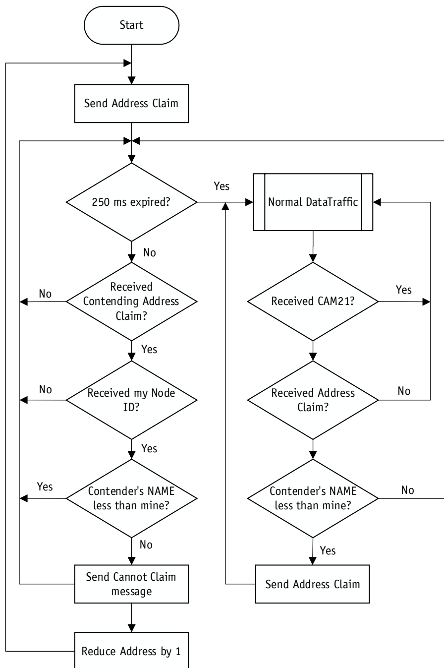
Fig. 3: Address Claiming
