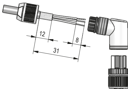
Fig. 11: Right angle mating connector M12
