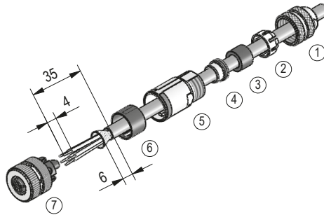
Fig. 10: Straight mating connector M12
