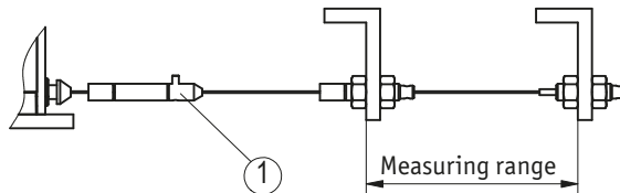
Fig. 8: Measuring range wire extension
