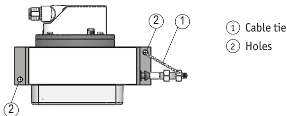
Fig. 3: Mounting
