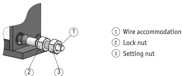
Fig. 4: Wire accommodation with thread
