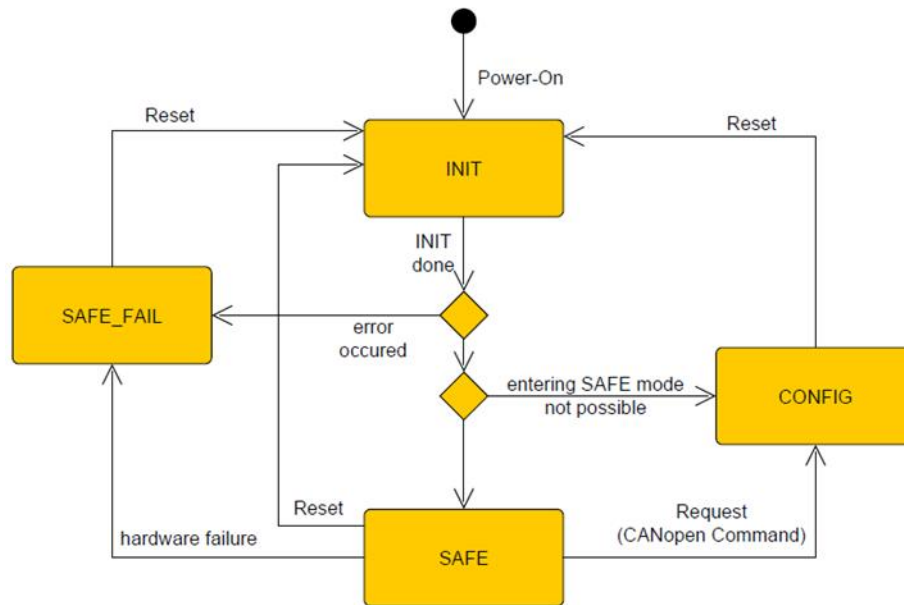
Fig. 18: Operating Mode State Machine
