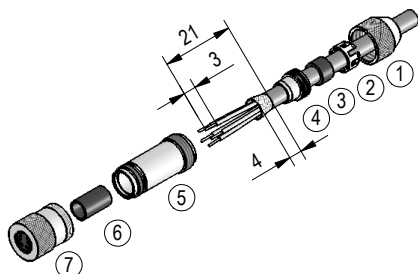
Fig. 15: Straight matting connector M12
