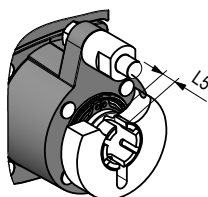
Fig. 6: Clamp ring, shaft with feather key groove
