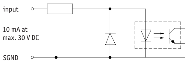
Fig. 9: input circuit
