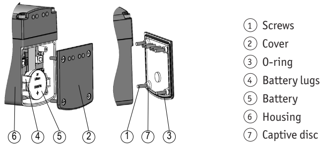
Fig. 14: Battery change
