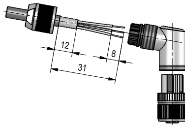
Fig. 16: Right angle mating connector M12
