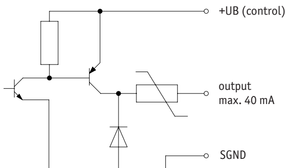
Fig. 8: output circuit
