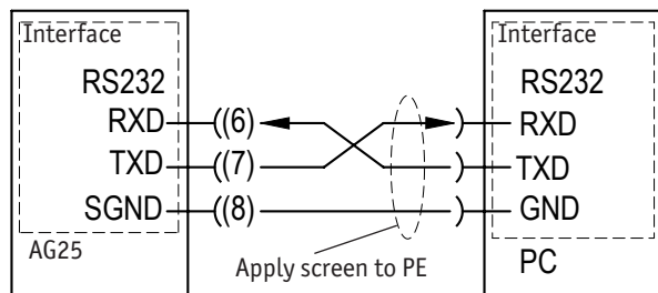
Fig. 10: Pinout schema RS232 interface
