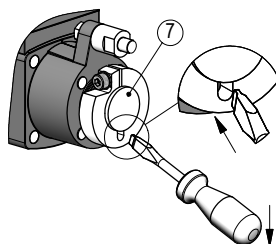
Fig. 5: Transport lock
