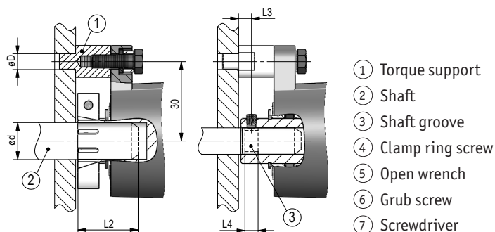
Fig. 1: Mounting dimensions
