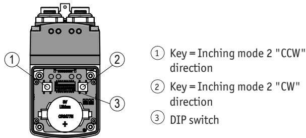
Fig. 13: Controls
