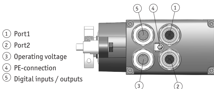
Fig. 7: Pin assignment
